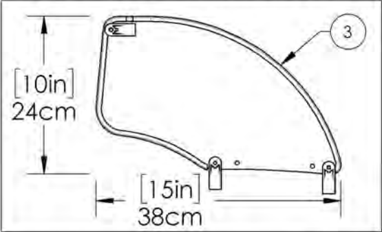
9001294 Side Guard - Carbon Fiber, Fixed, Left, Large
