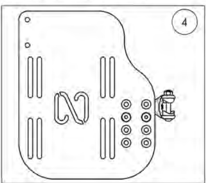
9002872 Footplate - Aluminium, Newton Angle Adjustable, Left, 7½ x 9½ in (Wheelchair Width: 19 in +)
