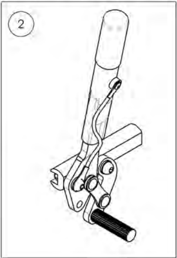
9001131 Wheel Lock - Pull to Lock, 6 in Removable Extension Handle, Left
