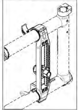
9001747 Rear Wheel Mounting Plate V2B - 6° Camber Angle
