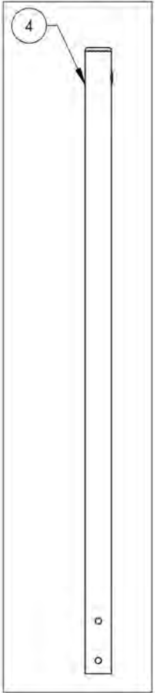
9001256 Back Cane - Carbon Fiber, Straight, Fixed 21 in
