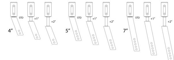
Frame length chart
